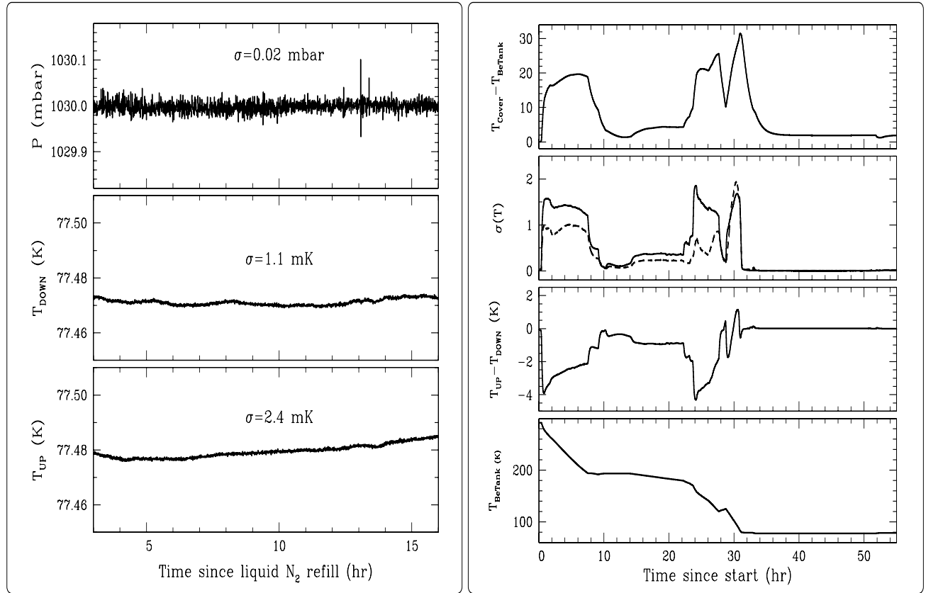
Figure 1. Left hand panel: variation of N 2 out-boiling pressure and BeTank temperature as a function of time since last refill, see Sect. 2 for details. Right hand panel: thermal behaviour of the system during a cooling cycle, see Sect. 3
