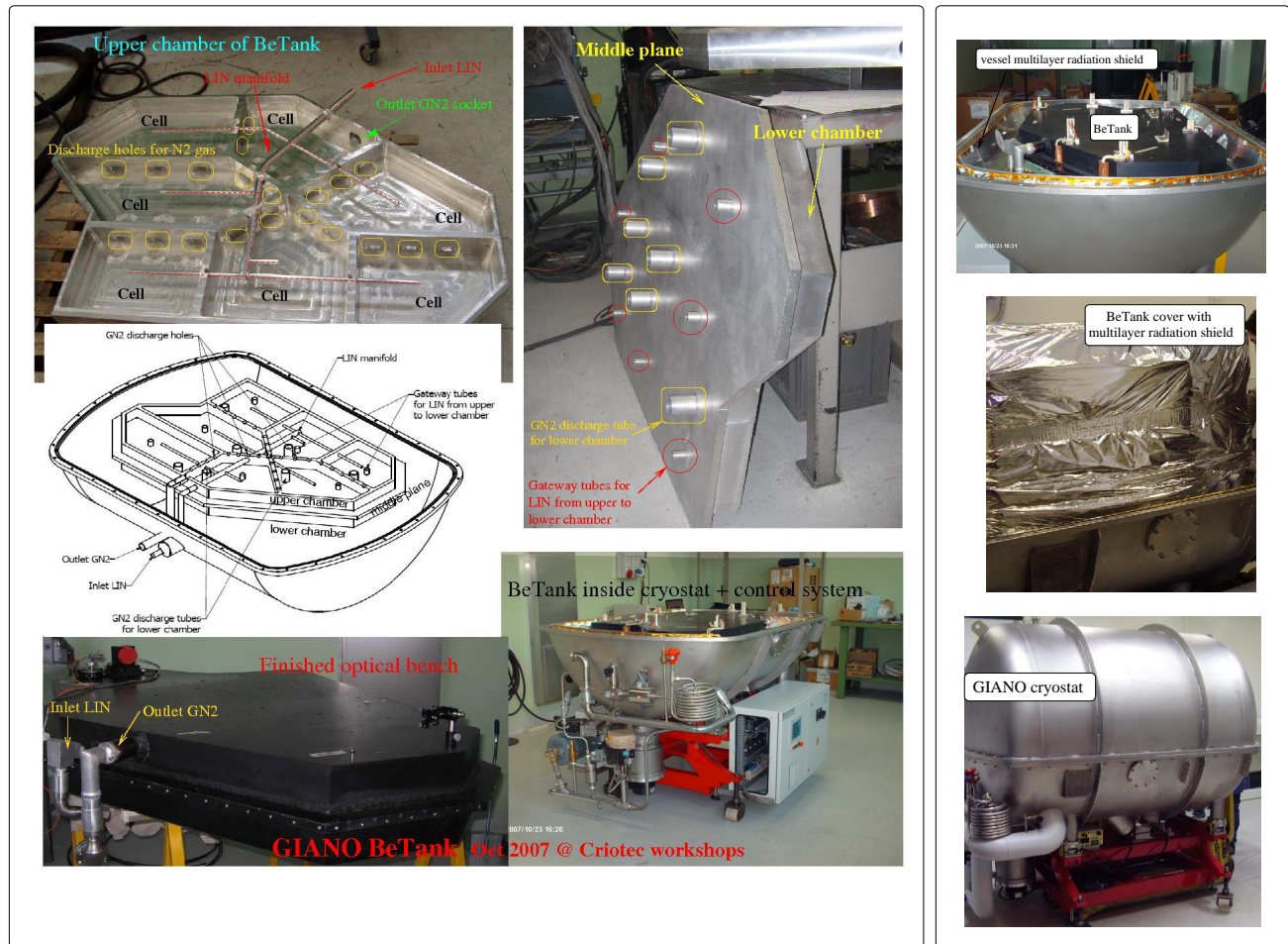
Figure 2. Left hand panel: design and pictures of the GIANO optical bench and liquid nitrogen tank (BeTank) during various phases of construction. The bottom right picture shows the system mounted inside the vacuum vessel and mounted on the structure which carries the cryogenic control system. Right hand panel: pictures of the GIANO cryostat (low), of the BeTank cover with its multilayer radiation shield (center) and of the BeTank together with the radiation shield mounted inside the vacuum vessel (top).
