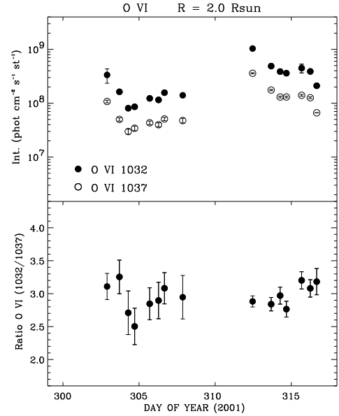
Figure 2. Top: total line-integrated intensities ( \text{ph cm}^{-2} \text{s}^{-1} \text{st}^{-1} ) for the 1032 (filled circles) and 1037 (open circles) Å lines of the O VI ion, vs. time, at 2 R_{\odot} , from UVCS observations. Bottom: ratio between the O VI \lambda 1032 and O VI \lambda 1037 line intensity, vs. time, at 2 R_{\odot} . Both panels give the 1\sigma error bars.
